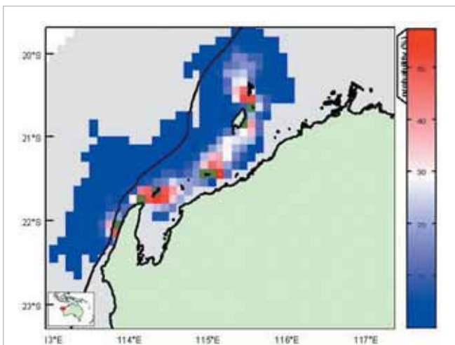
Figure 4. Connectivity statistics for a fish eggs and larvae sources indicated by the green squares, at Tandibiddi, Pt Murat (Ningaloo), Muiron Islands, Thevenard Island, Dugong Reef and Lowendal Shelf bommies after a 20 day dispersion in November (courtesy S Condie CSIRO).
