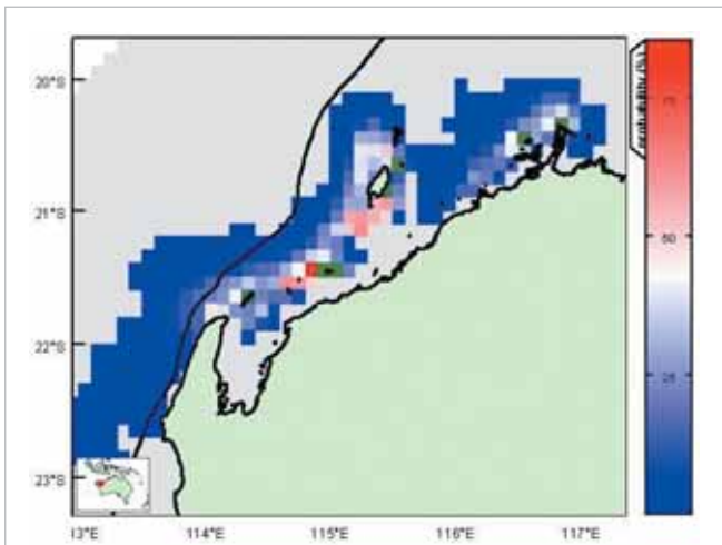
Figure 3. Connectivity statistics for coral spawn sources indicated by the green squares, at the Dampier Archipelago, Dugong Reef, Lowendal Shelf bommies and Thevenard Island, after a 20d dispersion in April. (courtesy S Condie CSIRO)
